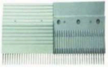
GEYNO: ES01KN1087 OEM: DEE1718891 Spec: 201.5 X173.5mm, Tooth Pitch 9, Hole Spacing153, 22T, Aluminum, Right
