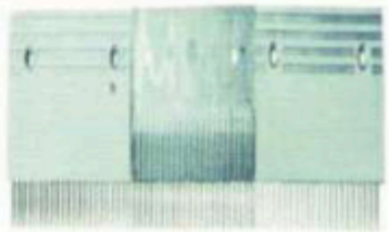
GEYNO: ES01KN1092 OEM: 5270418D10 Spec: 197.4 X162mm, Tooth Pitch 9, Hole Spacing140, 22T, Aluminum, Center
