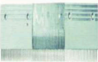
GEYNO: ES01KN1093 OEM: 5270417D10 Spec: 202.2 X162mm, Tooth Pitch 9, Hole Spacing140, 22T, Aluminum, Right
