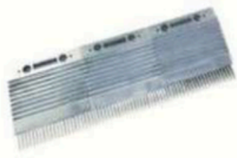
GEY NO: ES01KN1103 OEM: DEE2209590 Spec: RTV-C197,4X186.9mm, 22T, Aluminum
