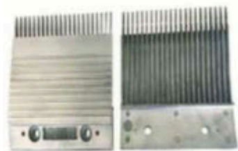
GEY NO: ES01KN1094 OEM: Spec: 197.4 X188.5mm, Tooth Pitch 9, Hole Spacing99, 22T, Aluminum, Center
