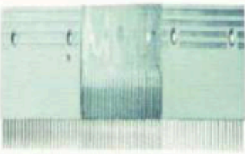
GEYNO: ES01KN1089 OEM: 5130669D10 Spec: 197.4 X127.2mm, Tooth Pitch 9, Hole Spacing140, 22T, Aluminum, Center
