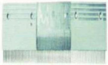
GEY NO: ES01KN1090 OEM: 5130668D10 Spec: 202.2 X127.2mm, Tooth Pitch 9, Hole Spacing140, 22T, Aluminum, Right
